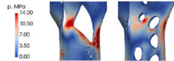
Stress distribution comparison between original and optimized design
