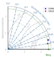
Figure 1: Comparison of metrics between the artificial intelligence model and the dynamic model (ECMWF) in the area of Galicia.
