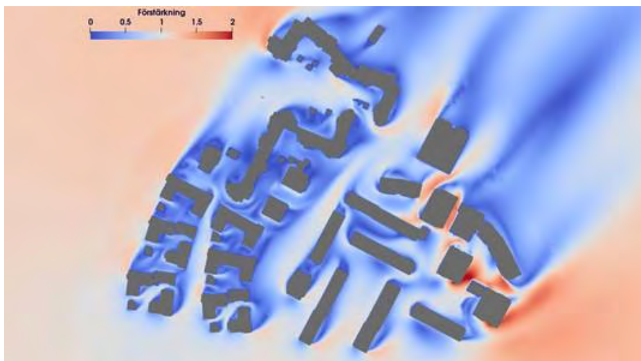
Figure 1: Example of a simulated air flow in an urban environment using OpenFOAM (method: RANS/k-epsilon). The amplification factor (color-coded) shows the wind velocity at two meters above ground level relative to a situation with wind over the same terrain without buildings, for wind from south-west.
