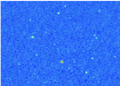
Figure 1: Output of the radio astronomy analysis pipeline, as run on the Canadian SKA regional node, showing clear sources of radio waves. © Tim Kok, SURF
