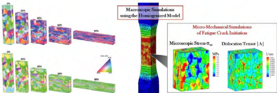
Figure 3: Example of crystal plasticity simulations (Damask software). Credits: Alleima AB.
