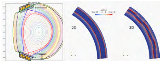
Figure 3: (left) Magnetic flux cross-section of WEST tokamak (right) Distribution of heat flux in \theta direction assuming constant magnetic field in \theta direction (2D magnetic field) and with varying magnetic field in \theta direction (3D magnetic field) where axisymmetry is broken and periodicity occurs, introducing higher level of complexity.
