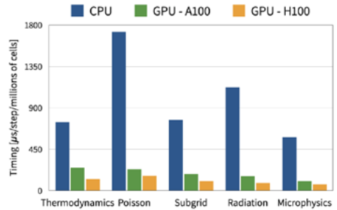
Figure 2: Timing comparison between CPU and GPU execution of DALES main physical processes, using a full Snellius AMD EPYC Genoa node vs. GPU nodes with 4 cards of the indicated type. The time step of the model is dominated by sequential subroutines that compute the effect of these processes.
