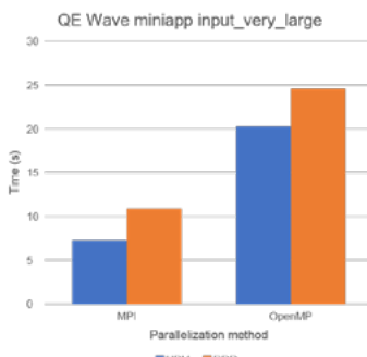
Figure 2: Execution time (in seconds) of Quantum Espresso mini-app on a single SNCA quadrant (i.e., 14 cores) of an Intel Sapphire Rapids processor equipped with both HBM and DDR, either by using only the HBM or only the DDR. The parallelization method used is either MPI (14 MPI process, 1 OpenMP thread per process) or OpenMP (1 MPI process, 14 OpenMP threads). © Eviden.
