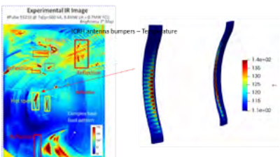
Figure 4: (left) Experimental IR camera image in WEST tokamak. 2 Temperature distribution on ICRH antenna bumpers by solving first two steps of the workflow: field-line tracing and thermal model. The result matches experimental result to some level of degree.
