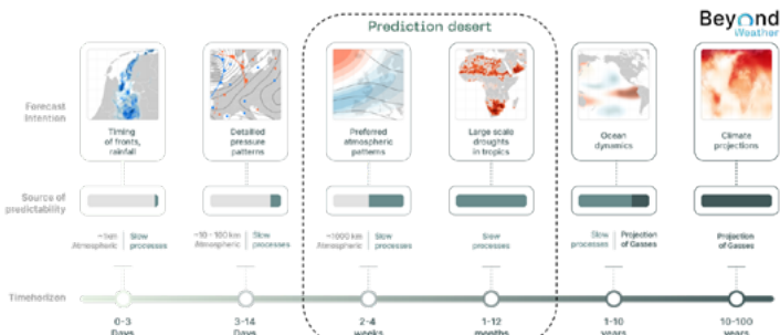
Figure 1: The challenge, predicting weather beyond 2 weeks is notoriously difficult. © 2024 Beyond Weather
