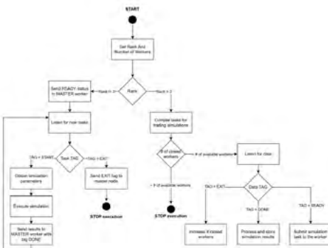
Figure 1: Orchestration of trading simulations for multinode multicore environment
