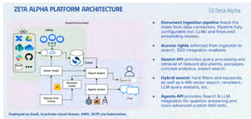
Figure 2: Zeta Alpha platform architecture @ 2024 Zeta Alpha
