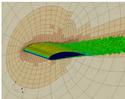
Figure 3: Vortical structures for the flow around a periodic wing. Structure of the AMR mesh is presented by black lines (element interfaces) and a colourmap showing various refinement levels.
