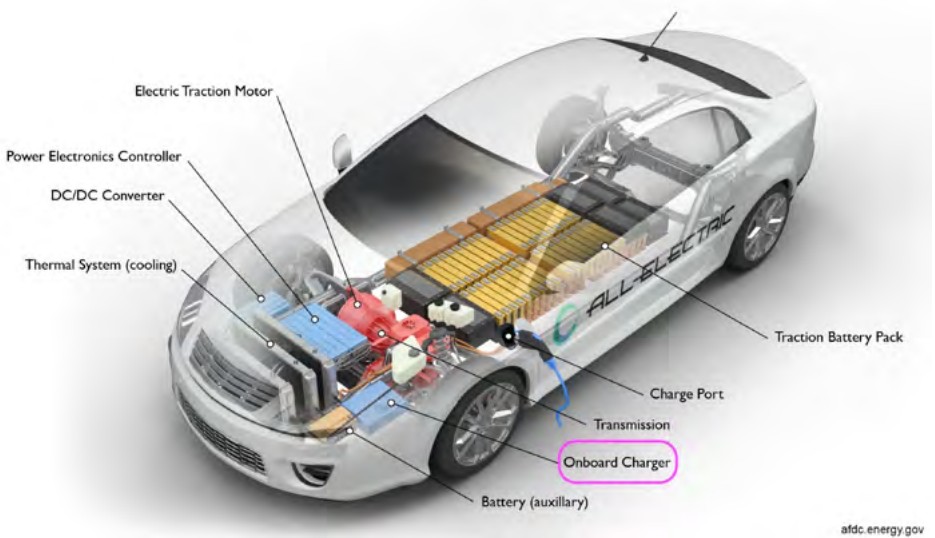
Figure 1: Key Components of an All-Electric Car Image source: https://afdc.energy.gov/vehicles/how-do-all-electric-cars-work Illustration identifying various components involved in the project.
