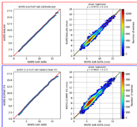
Figure 1: Comparison of metrics between the artificial intelligence model and the dynamic model (ECMWF) in the area of Galicia.
